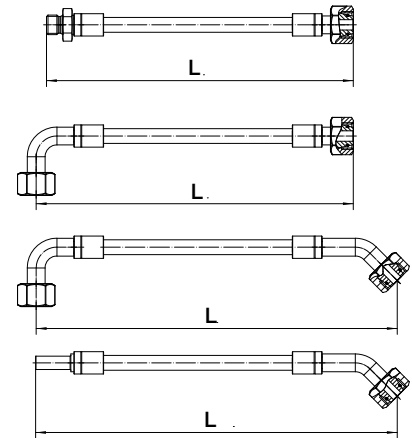
Figure 8: An illustration showing how to measure the length of hose assemblies correctly
